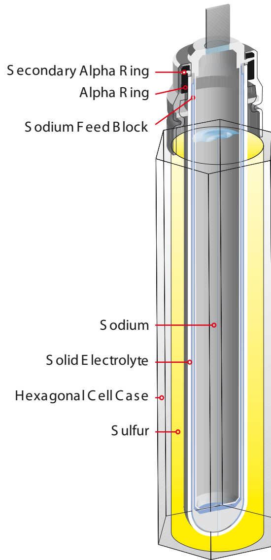
Fig. 4: Hexagonal Cell
